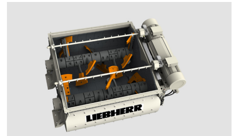
Twin-shaft mixer of a concrete mixing plant, rendered with KeyShot
